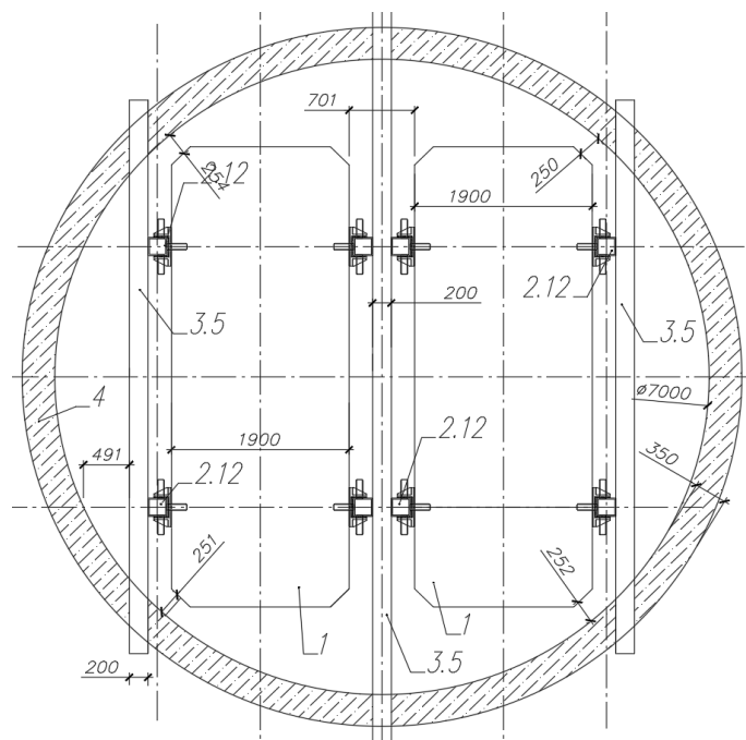
1 - lifting vehicle (cage of 2KN4-2 type); 2.12 – rigid guide; 3.5 – rigid buntun; 4 - shaft lining; 7 - anchor
